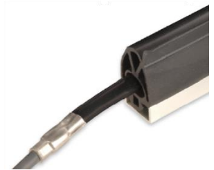
ENT-7 assembly with end piece ENES-Kx in rubber profile
