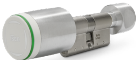
Libra X Smart electronic modular cylinder with RFID/Bluetooth reader and Standard mechanical knob.
